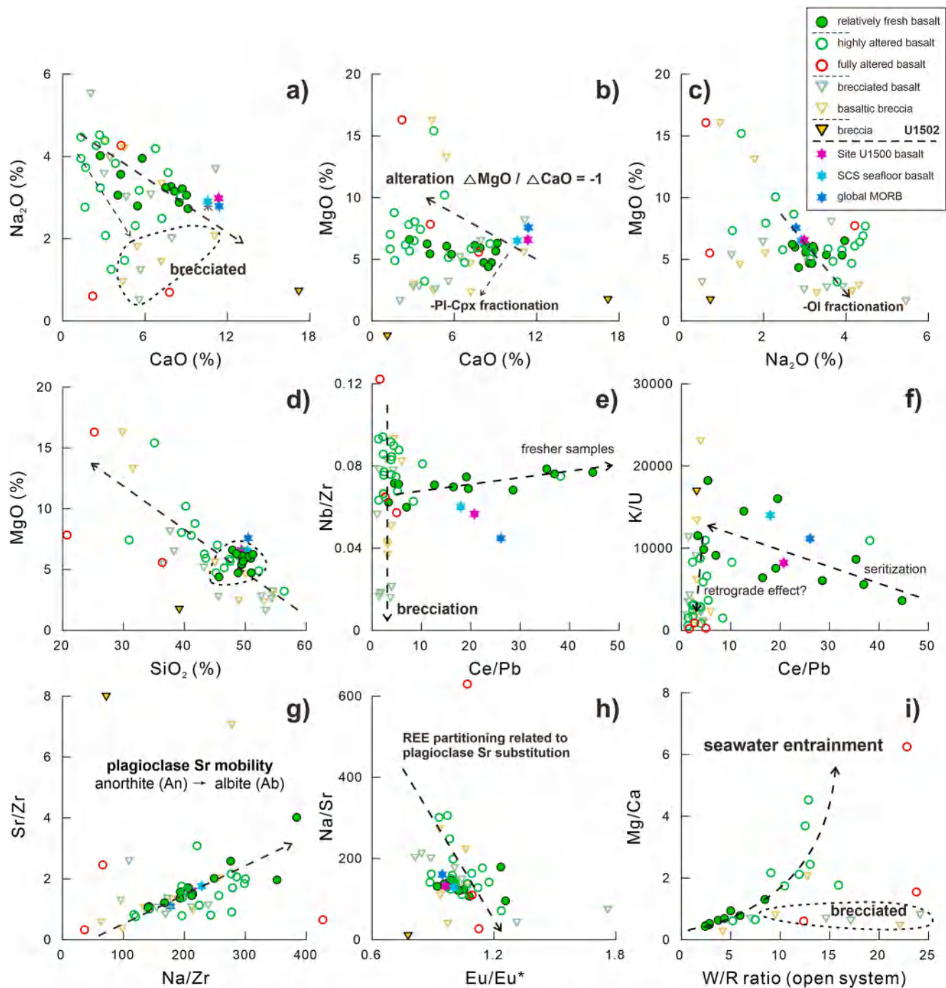
Fig. 9. Plots of diagnostic proxies for the hydrothermal processes occurred in the basaltic rocks of IODP Hole U1502B. For the sample-types of Hole U1502B see Fig. 2. Sources of reference data refer to the caption of Fig. 3. For interpretations see Sections 6.1 and 6.2.
