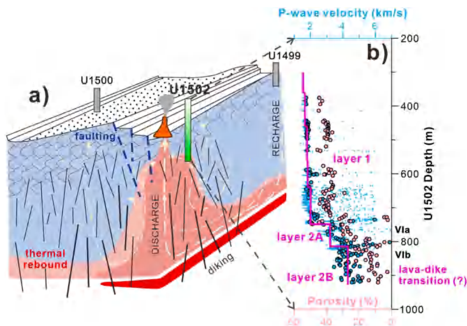
Fig. 11. Schematic model for fluid-rock reaction within the upper crust of the northern SCS rift margin (after Coogan, 2008; Sun et al., 2019) (a), showing the data of P-wave velocity and crustal porosity for Site U1502 (after Larsen et al., 2018b; Ding et al., 2020) (b). Hole U1502B should have penetrated the boundary of seismic layer 2A/2B, likely related to an alteration front of hydrothermal circulation and/or the lithologic lava-dike transition. As triggered by the large detachment fault inland of COT, multiple normal faulting developed along with the widespread dikes and sills, providing the ascending channels for hydrothermal fluids during the SCS rifting. Within the variable environments of discharge zone, a two-stage migration is thought to produce the alteration effects as observed in Hole U1502B. Our scenario explains the differences on crustal structure and hydrothermal alteration between Sites U1499, U1500, and U1502, underlining the tectonic effects imposed by detachment-related faulting. For interpretations see Section 6.3.
