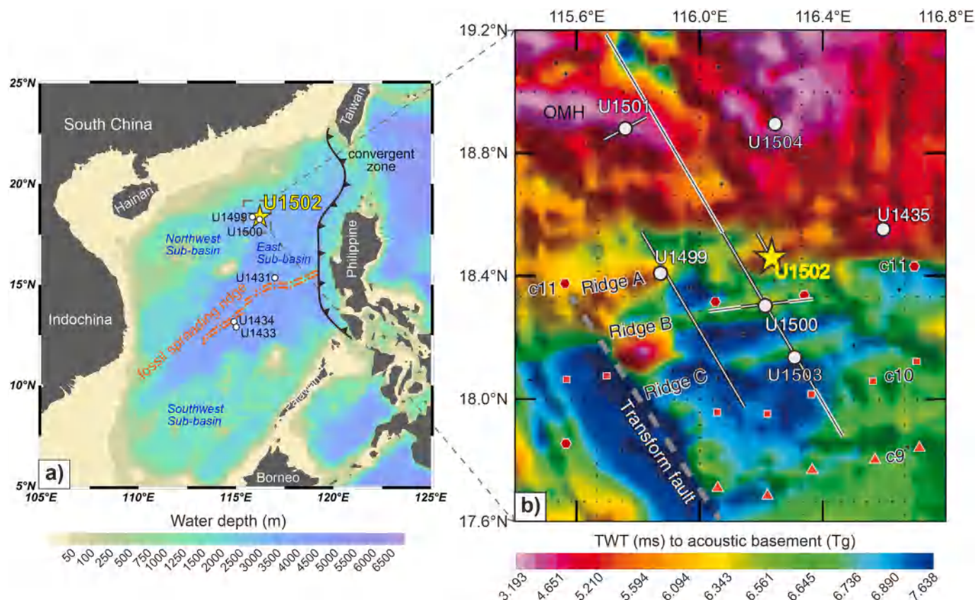
Fig. 1. Geological setting of the continent–ocean transition (COT) zone in the northern margin of the South China Sea (SCS), showing the locations of IODP Site U1502 (yellow star) and other IODP sites mentioned in text (gray circles). a) Bathymetric map of the modern SCS, with tectonic features and three sub-basins indicated. b) Two-way traveltime (TWT) depth to the Tg acoustic basement, revealing the key basement topography: Outer Margin High (OMH) and the distinct Ridges A, B, and C (for seismic lines and profiles see Jian et al., 2018; Sun et al., 2018). Magnetic anomalies (C9, C10, and C11; red symbols) are also depicted (after Briaies et al., 1993; Larsen et al., 2018a). Note that the oldest picked magnetic Chron C11n ( \sim 30 Ma) is between the Ridges A and B, seaward of Site U1502. For details see Section 2. (For interpretation of the references to color in this figure legend, the reader is referred to the web version of this article.)
