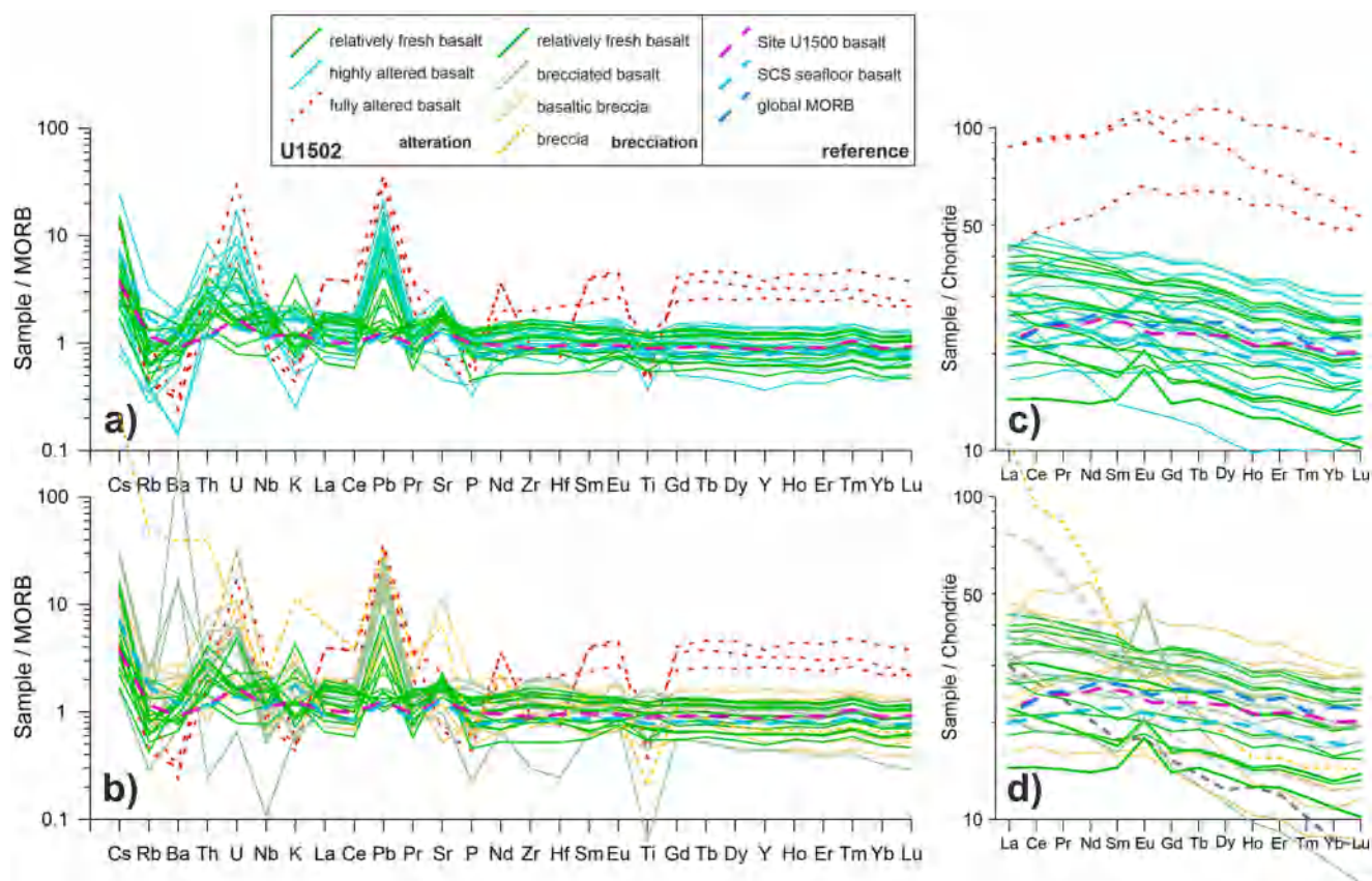
Fig. 5. Trace element patterns for the hydrothermally altered basaltic rocks of IODP Hole U1502B: incompatible element patterns normalized to global MORB (Gale et al., 2013), arranged in the order of ascending compatibility (Sun and McDonough, 1989) (left panel); and REE (i.e. rare earth element) fractionation patterns with normalization to chondrite (Anders and Grevesse, 1989) (right panel). Comparisons of the relatively fresh basalts with the samples affected by hydrothermal alteration alone (a, c), and with the samples also affected by hydro-fracturing brecciation (b, d). Sources of reference data refer to the caption of Fig. 3.
