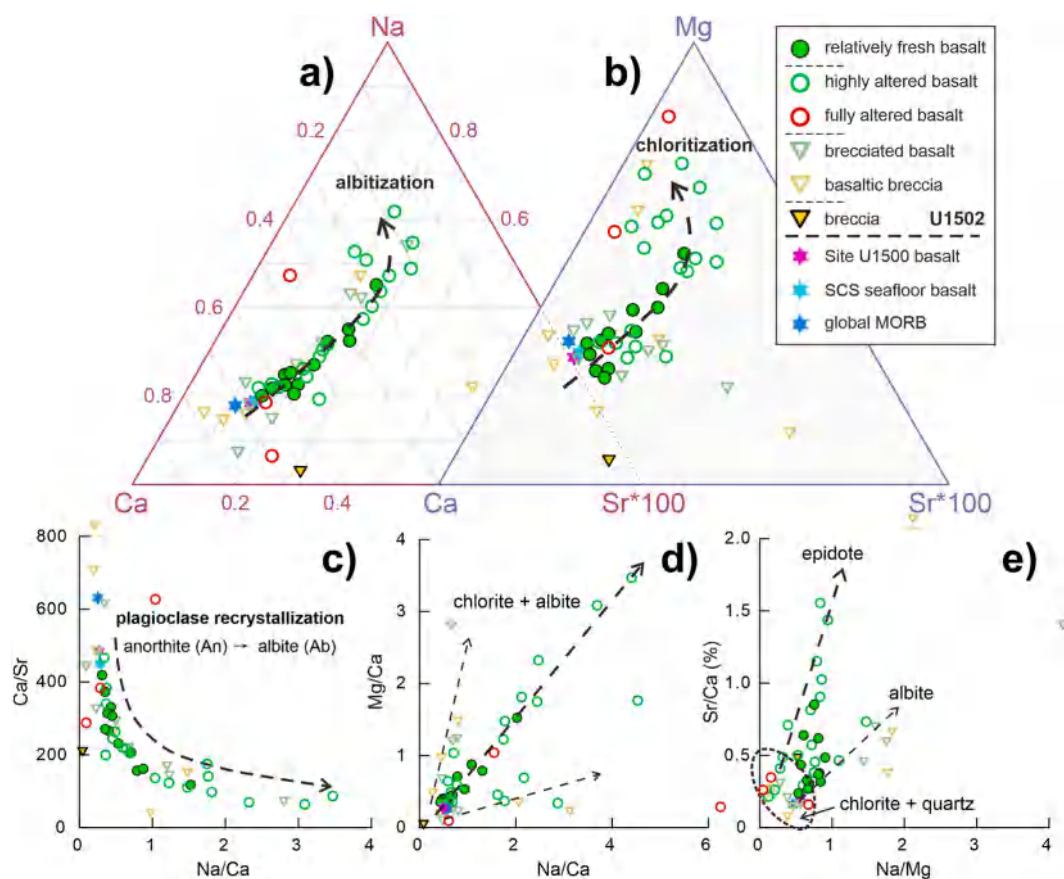
Fig. 10. Correspondences between Ca, Na, Mg, and Sr contents reveal the plagioclase-regulated alterations in the basalt sequence of IODP Hole U1502B. For different kinds of samples, the tight Ca–Sr–Na relationship indicates the major role of albitization on the Ca loss (a, c). The similar trend of Ca–Sr–Mg space but more scattered data reflect the exchange of seawater Mg for basaltic Ca through the transformation of plagioclase to chlorite, and a facilitating role of chloritization on albitization (b, d). Albite formation causes little/no change in Sr but is characterized by enhanced Na/Ca ratio; chlorite formation corresponds to the trends with increasing Mg and decreasing Sr; and primary plagioclase replaced by epidote leads to whole-rock Sr enrichment (c–e). For the sample-types of Hole U1502B see Fig. 2. Sources of reference data refer to the caption of Fig. 3.
