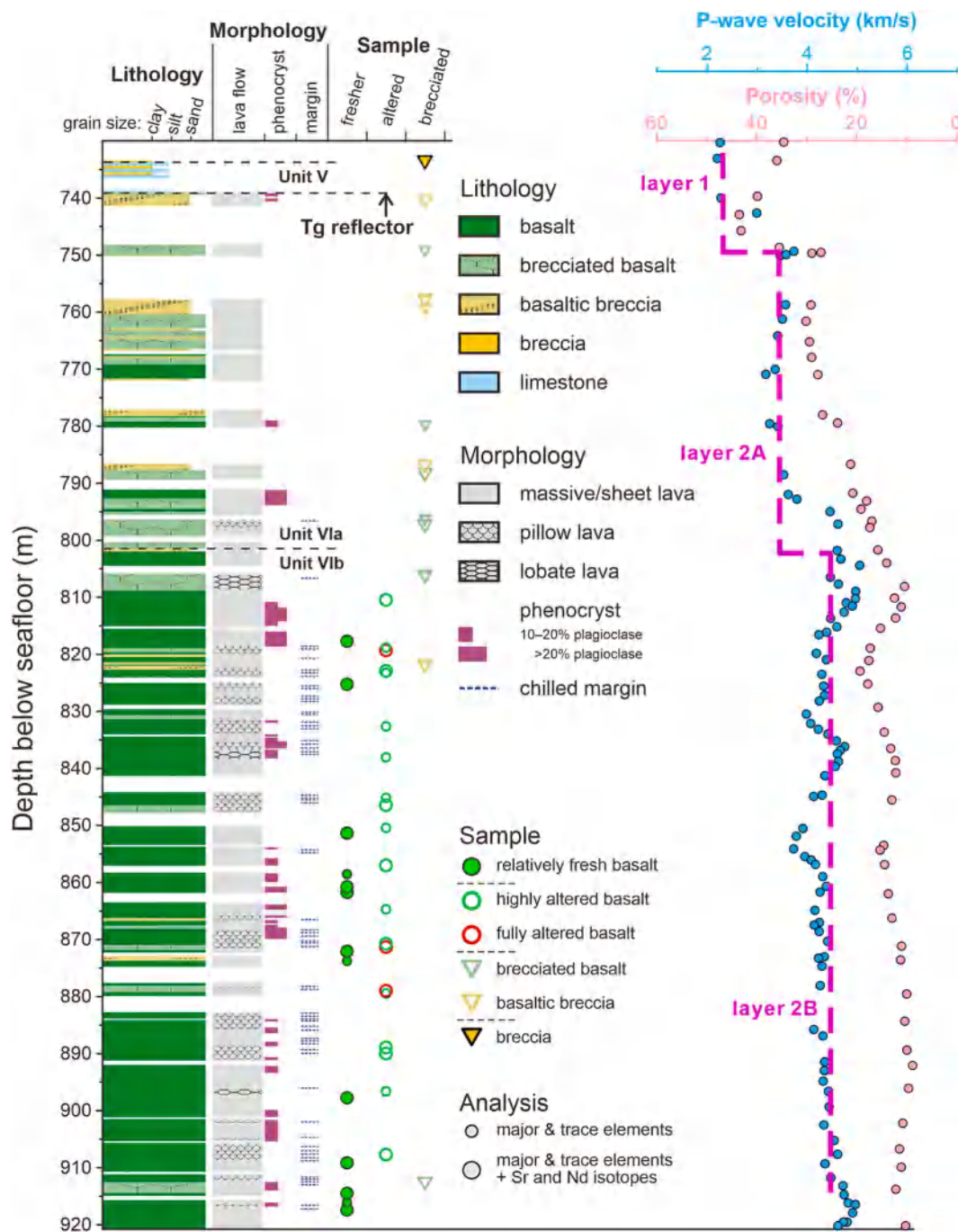
Fig. 2. Lithostratigraphy of IODP Hole U1502B, with the sampled intervals shown (after Larsen et al., 2018b). Separated from sedimentary Unit V by the Tg reflector, igneous Unit VI is divided into VIa and VIb sub-units, according to the lithology, flow morphology, and alteration style/intensity. The lithologies consist mainly of basalt, brecciated basalt, basaltic breccia, overlain by minor breccia and limestone. The morphology of lava-flow are distinguished between massive/sheet, pillow, and lobate, with the intervals of highly phryic basalts (i.e. >10% plagioclase phenocrysts) and chilled margins specified. A total of 50 whole-rock samples are categorized into 6 types based on petrographic inspections (Table S1; Figs. S1–S4), consistent with the Proceedings of IODP Expeditions 367/368 (Jian et al., 2018; Sun et al., 2018). All samples were analyzed for geochemical composition (Datasets S1–S3), and a selection of 30 samples (larger symbols) were measured for Sr and Nd isotopes (Dataset S4). In right panel, the data of P-wave velocity (caliper data) and porosity (with inverse axis) are shown as 5-point moving average (Larsen et al., 2018b). Notably, the concurrent trends of P-wave velocity and crustal porosity data may indicate the seismic stratigraphy of Hole U1502B in the upper oceanic crust (i.e. penetration into the layer 2A/2B; also see Fig. 11). For details see Sections 3 and 4 and Supporting Information.
