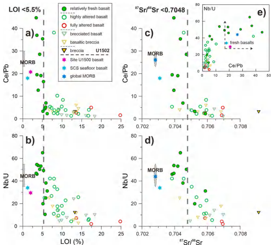
Fig. 6. Close correspondences with LOI and ^{87}\text{Sr}/^{86}\text{Sr} data permit the use of Ce/Pb and Nb/U ratios as reliable proxies of alteration degree in IODP Hole U1502B. The basalt samples that were not apparently affected by hydrothermal alteration are identified, i.e. those with LOI <math>< 5.5\%</math> and ^{87}\text{Sr}/^{86}\text{Sr} < 0.7048 . For the sample-types of Hole U1502B see Fig. 2. Sources of reference data refer to the caption of Fig. 3.
