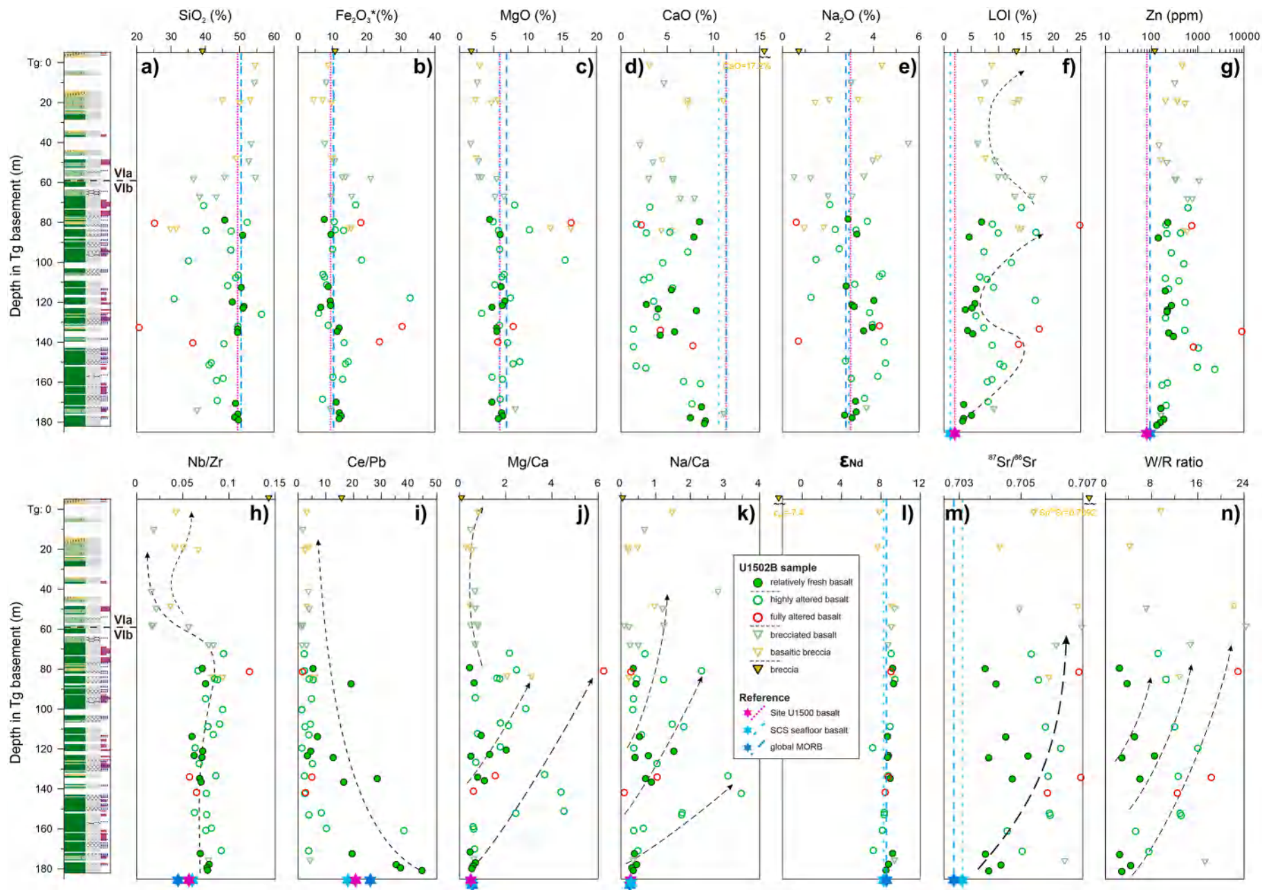
Fig. 3. Downhole profiles of selected proxies for the hydrothermally altered basaltic rocks of IODP Hole U1502B. Lithostratigraphy is shown relative to the Tg reflector (i.e. in oceanic basement; see Fig. 2), and different types of samples are distinguished (see Section 3). \text{Fe}_2\text{O}_3^* refers to total iron oxides; the data of loss on ignition (LOI) and the water/rock (W/R) ratio estimated from Sr isotopes systematics are also plotted. For reference, the SCS basalts sampled by IODP Expeditions 367/368 on the same rifted margin (Sites U1500; Yu and Liu, 2020), and by Expeditions 349 on the spreading seafloor (Sites U1431, U1433, and U1434; Zhang et al., 2018) are compared (see Fig. 1), in addition to the global MORB (Gale et al., 2013).
