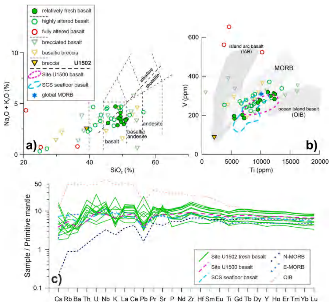
Fig. 4. Geochemical discrimination for the protolith of IODP Hole U1502B: a) plot of total alkalis (Na 2 O + K 2 O) vs. SiO 2 (Macdonald and Katsura, 1964); b) plot of V vs. Ti (Shervais, 1982), compared with the reference data of MORB (Gale et al., 2013), IAB (Labanih et al., 2012), and OIB (Chauvel et al., 2011); and c) incompatible element pattern normalized to primitive mantle (Sun and McDonough, 1989). For the sample-types of Hole U1502B see Fig. 2. Sources of reference data refer to the caption of Fig. 3.
