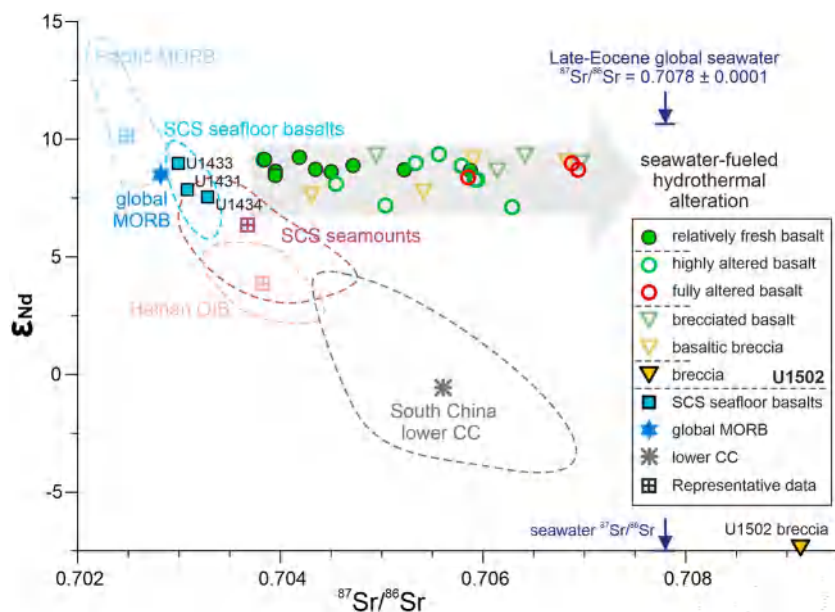
Fig. 7. Plot of \epsilon_{\text{Nd}} vs. ^{87}\text{Sr}/^{86}\text{Sr} of the hydrothermally altered basaltic rocks of IODP Hole U1502B. Sources of the reference data: SCS seafloor basalts (i.e. Sites U1431, U1433, and U1434; Zhang et al., 2018), global and Pacific MORB (Gale et al., 2013), and lower CC (i.e. lower continental crust) of South China (Dai et al., 2008); and averaged data of Hainan OIB (after Zhang et al., 2018) and SCS seamounts (after Zhong et al., 2018). Variations in ^{87}\text{Sr}/^{86}\text{Sr} point to a pervasive hydrothermal alteration, which has little affected the mantle-derived, nearly invariable \epsilon_{\text{Nd}} values. The hydrothermal fluids appear to evolve in ambient seawater of late-Eocene age (global seawater ^{87}\text{Sr}/^{86}\text{Sr} signature: 0.7078 \pm 0.0001 ; McArthur et al., 2012).
